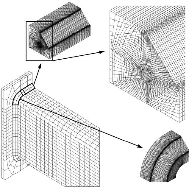
Fig. 5.21: Overall model and sub-models of Participant A
