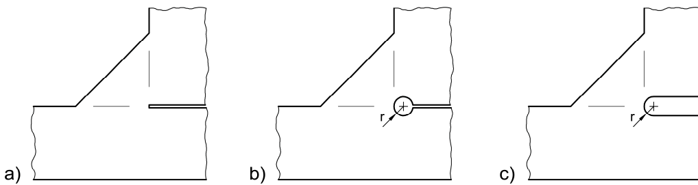
Fig. 3.2: Rounding of the weld root of a non-penetrating fillet weld by a keyhole and an U-shaped notch
