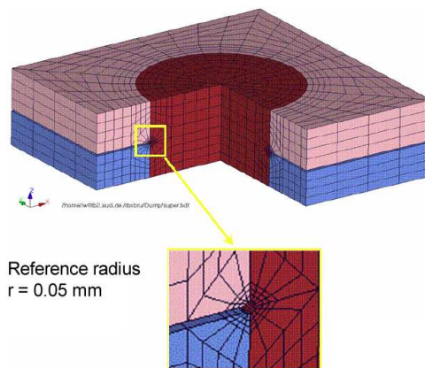
Fig. 5.24: Super-element of a spot-weld with reference radius r_{\text{ref}} = 0.05 \text{ mm} (de Bruyne and Hoppe, 2006)
