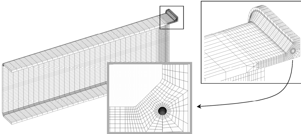
Fig. 5.16: Finite element model of Participant B
