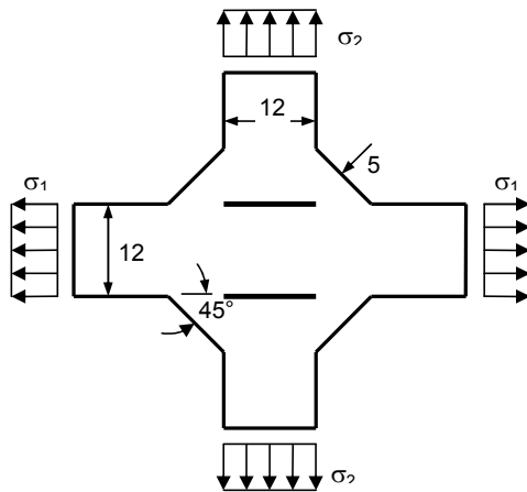
Fig. 5.1: Fillet welded cruciform joint
