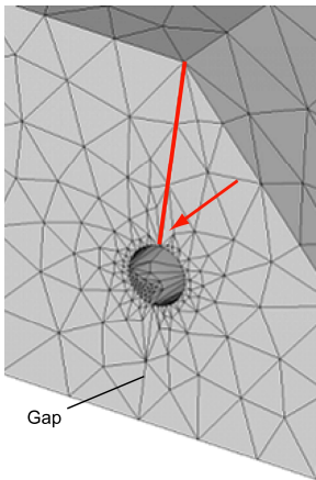
Fig. 5.19: Local mesh of Participant G
