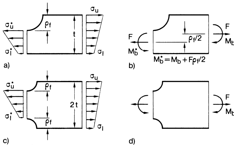
Fig. 3.9: Modification of the membrane and bending stress by fictitious notch rounding with undercut at one side (a,b) or at both sides (c,d), after Radaj et al. (2006)
