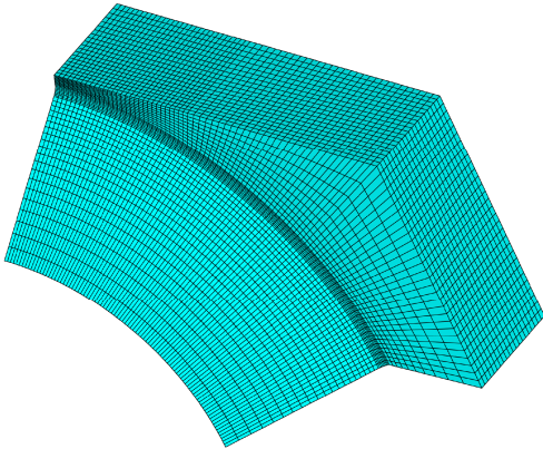
Fig. 5.12: Sub-model of critical area (Participant A)
