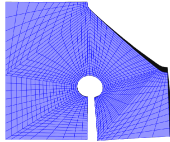
Fig. 5.22: Deformation of the sub-model for bending load
