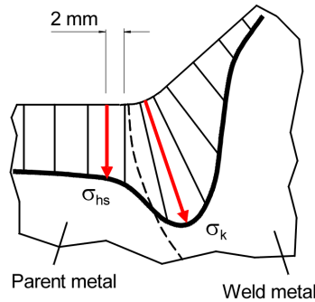
Fig. 4.3: Stress distribution at a weld toe
