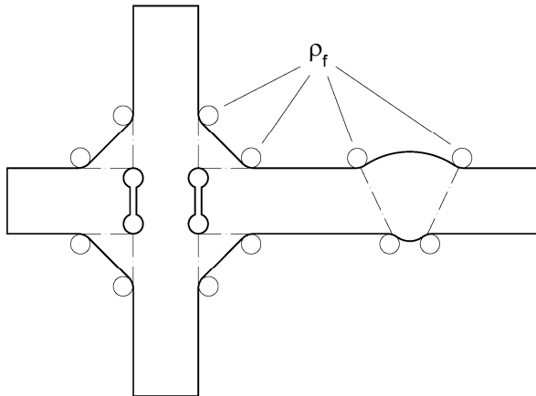
Fig. 2.1: Fictitious notch rounding (graph according to Hobbacher, 1996)
