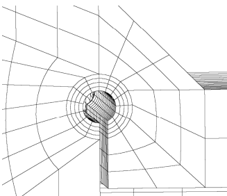
Fig. 5.17: Local mesh of Participant E
