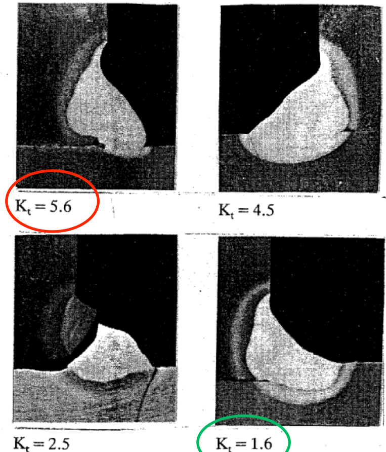
Fig. 6. Weld geometries and computed K_t .
